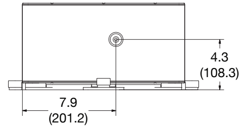
Input End View
